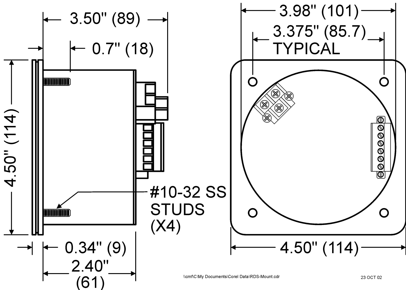
Figure 1 – Instrument Dimensions
